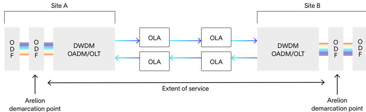
Wavelengths network components
